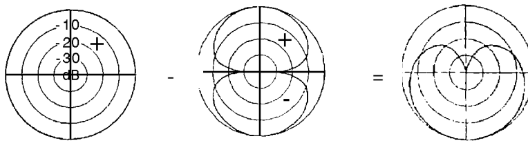
W signal minus X signal equals reversed cardioid
