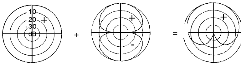
W signal plus X signal equals cardioid
